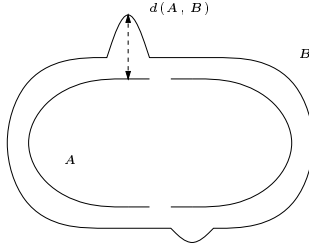
Figure 6: Hausdorff distance.
